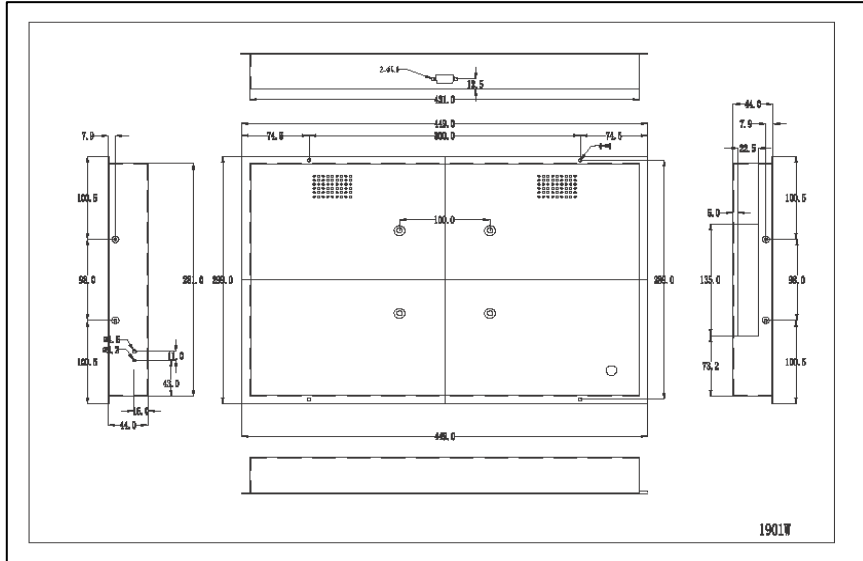
Mechanical Drawing
